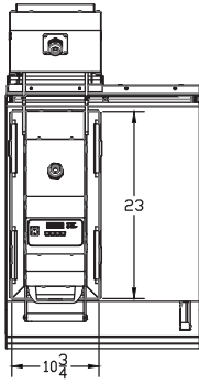
TOP VIEW
