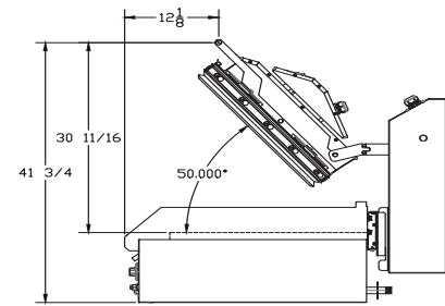
SIDE VIEW : TILTED
